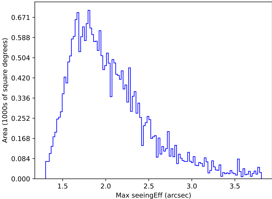
weather_cloudso14v3.4_10yrs Yr 1 all bands: Max seeingEff
