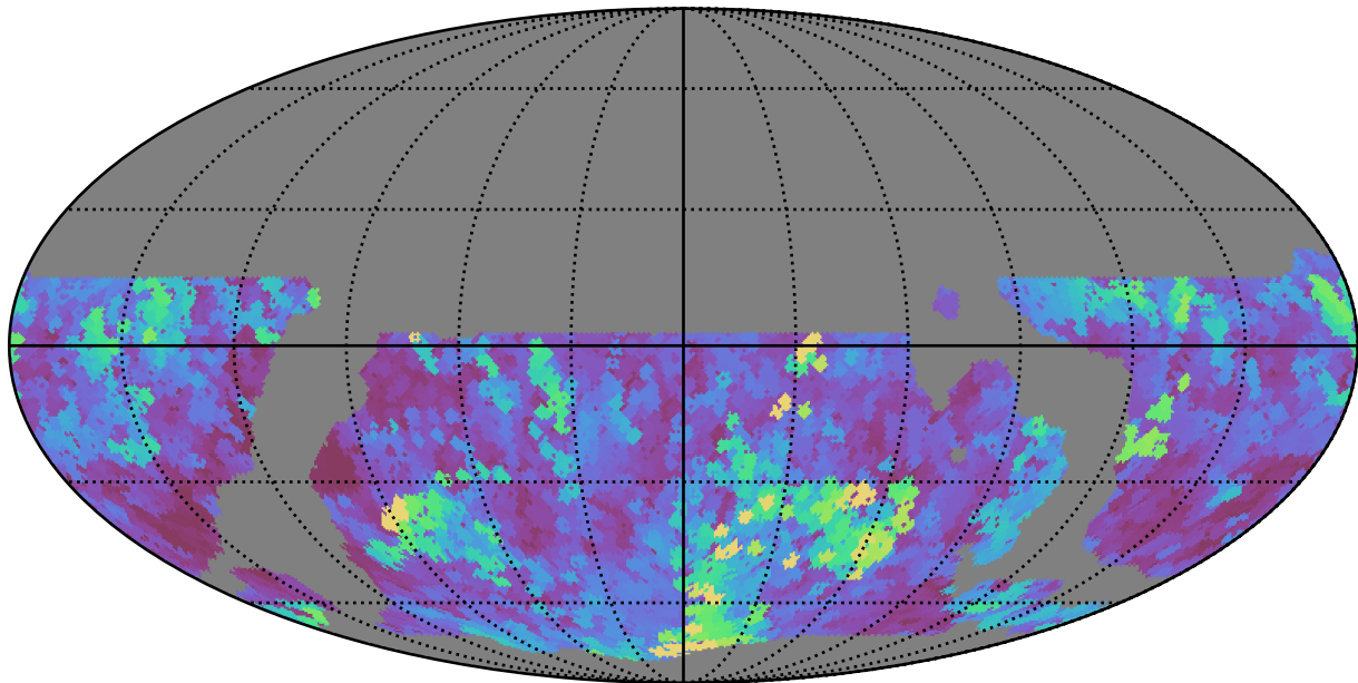
weather_cloudso14v3.4_10yrs WFD z band: Max seeingEff
