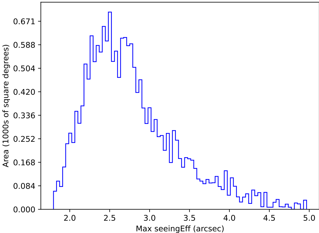
weather_cloudso14v3.4_10yrs WFD z band: Max seeingEff
