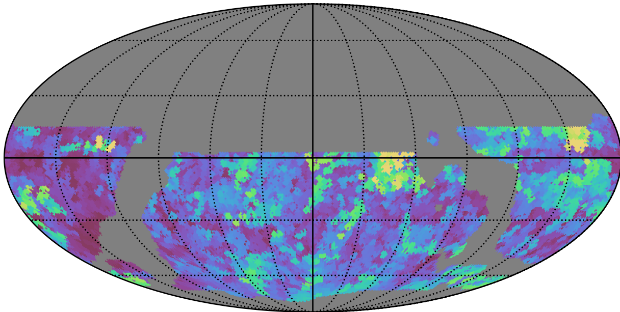
weather_cloudso14v3.4_10yrs WFD r band: Max seeingEff
