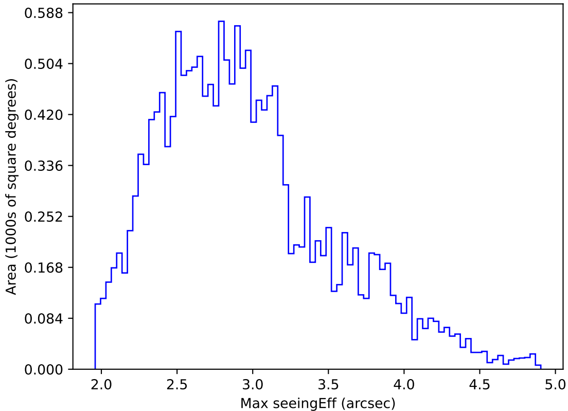
weather_cloudso14v3.4_10yrs WFD r band: Max seeingEff
