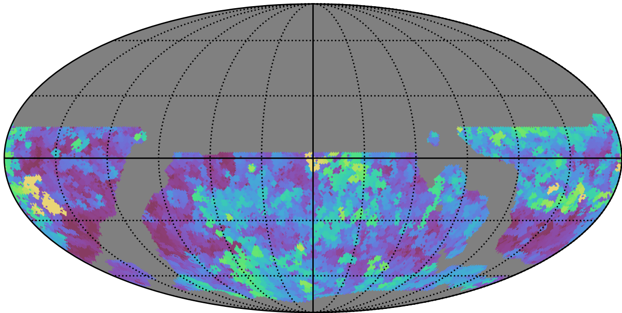
weather_cloudso14v3.4_10yrs WFD g band: Max seeingEff
