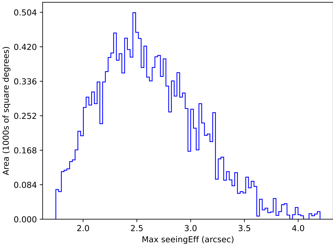
weather_cloudso14v3.4_10yrs WFD g band: Max seeingEff
