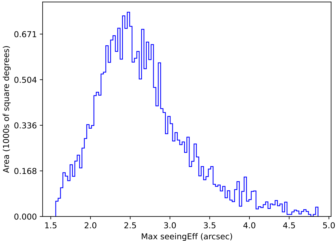
weather_cloudso14v3.4_10yrs All sky z band: Max seeingEff
