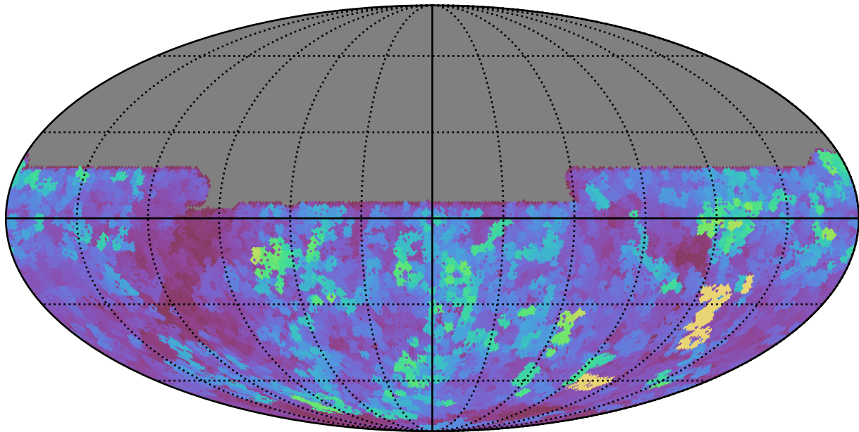
weather_cloudso14v3.4_10yrs All sky y band: Max seeingEff
