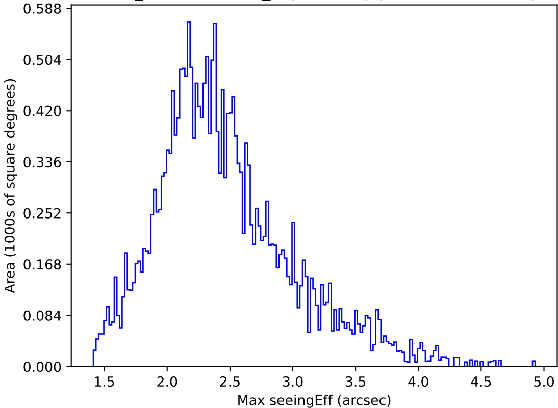
weather_cloudso14v3.4_10yrs All sky y band: Max seeingEff
