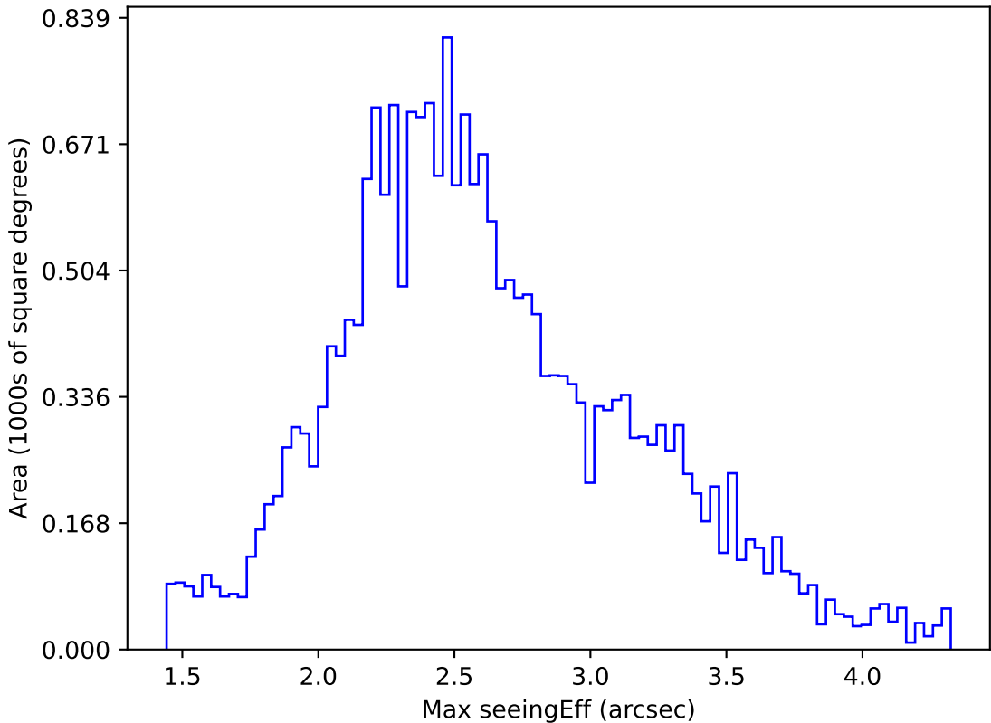
weather_cloudso14v3.4_10yrs All sky u band: Max seeingEff
