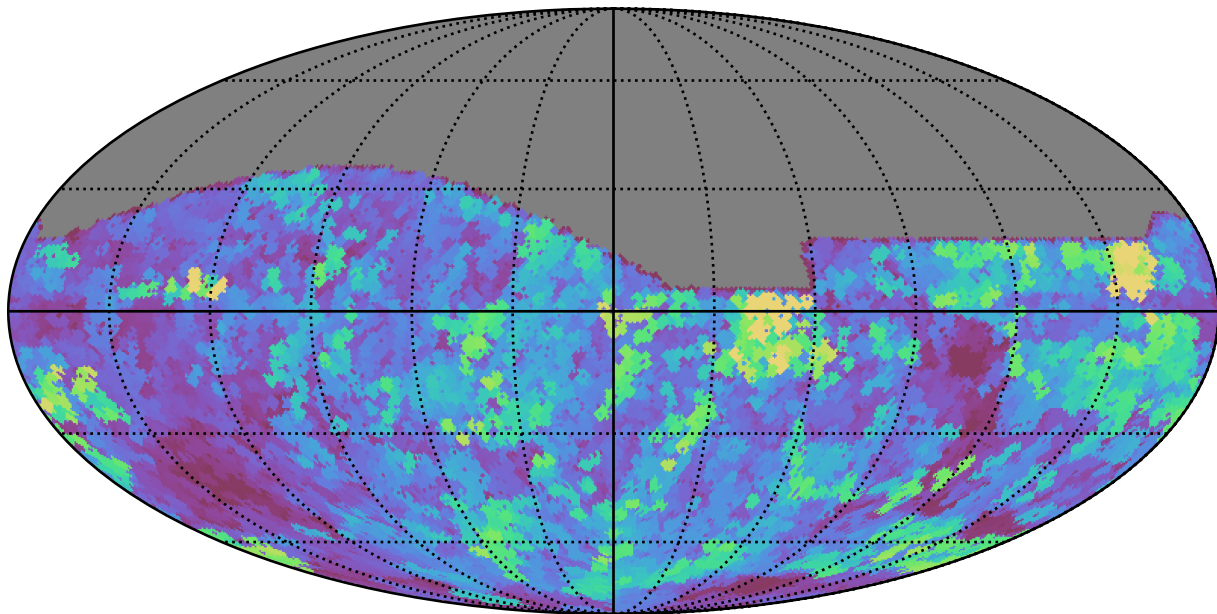
weather_cloudso14v3.4_10yrs All sky r band: Max seeingEff
