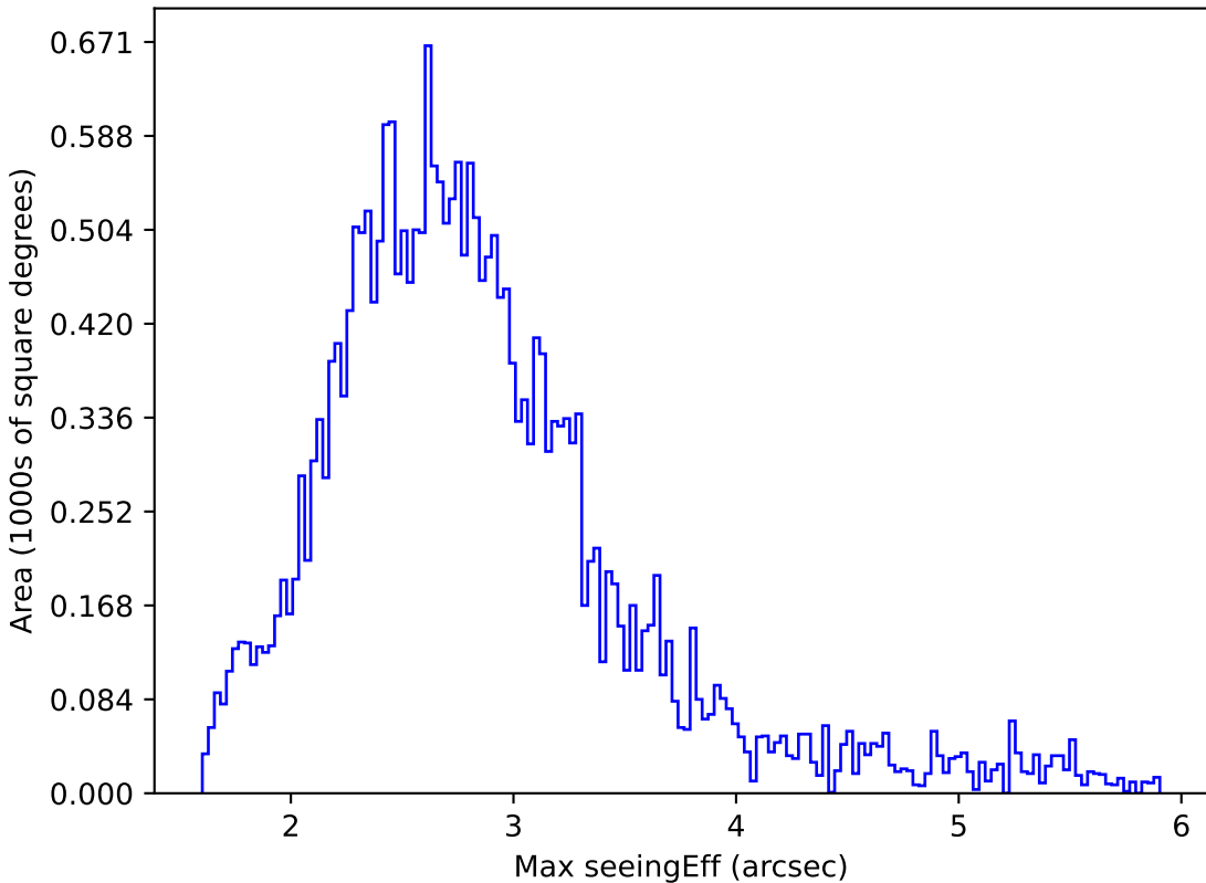
weather_cloudso14v3.4_10yrs All sky i band: Max seeingEff
