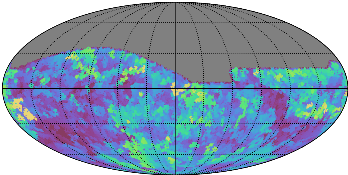
weather_cloudso14v3.4_10yrs All sky g band: Max seeingEff
