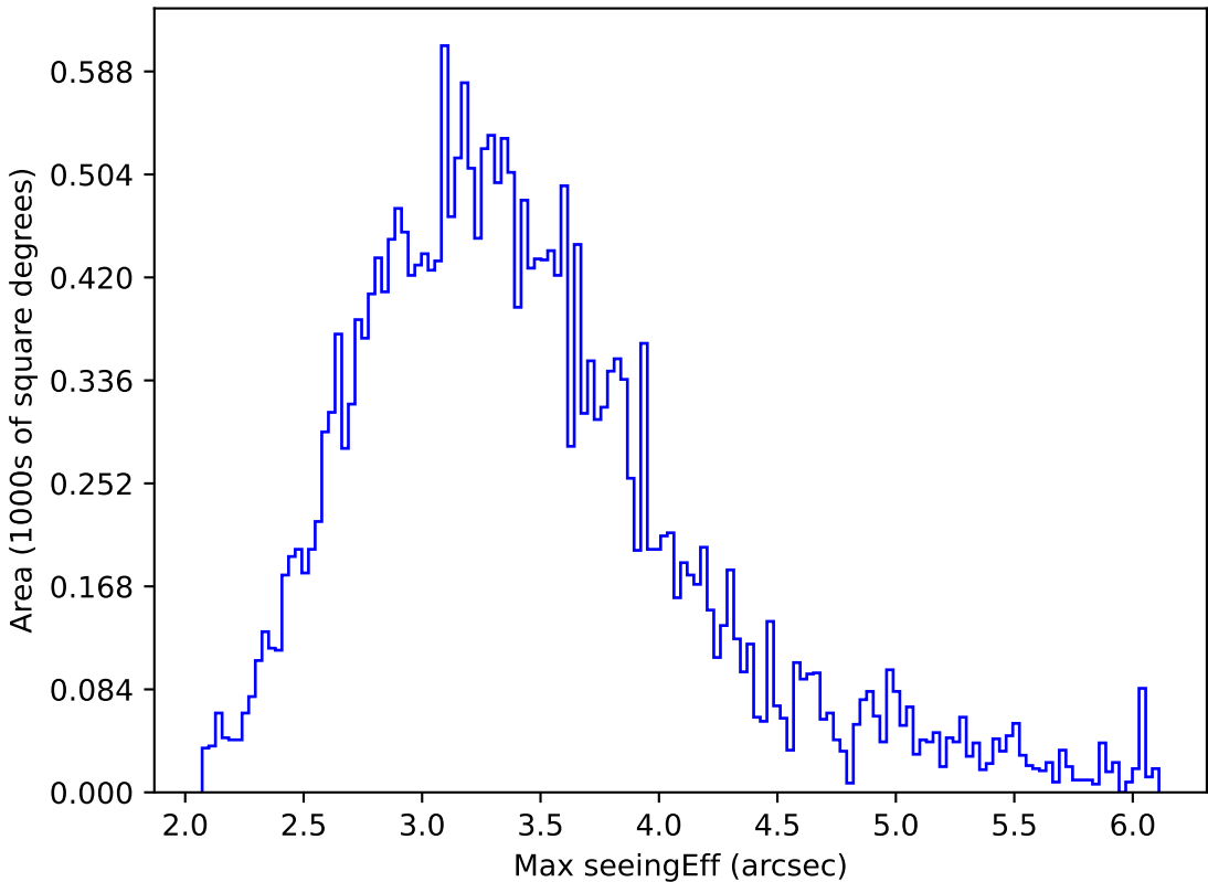
weather_cloudso14v3.4_10yrs All sky all bands: Max seeingEff
