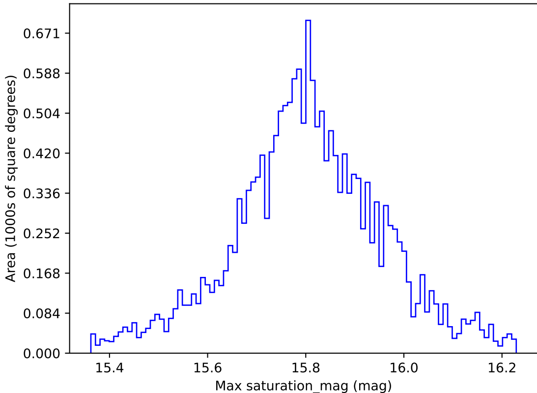
weather_cloudso14v3.4_10yrs WFD all bands: Max saturation_mag
