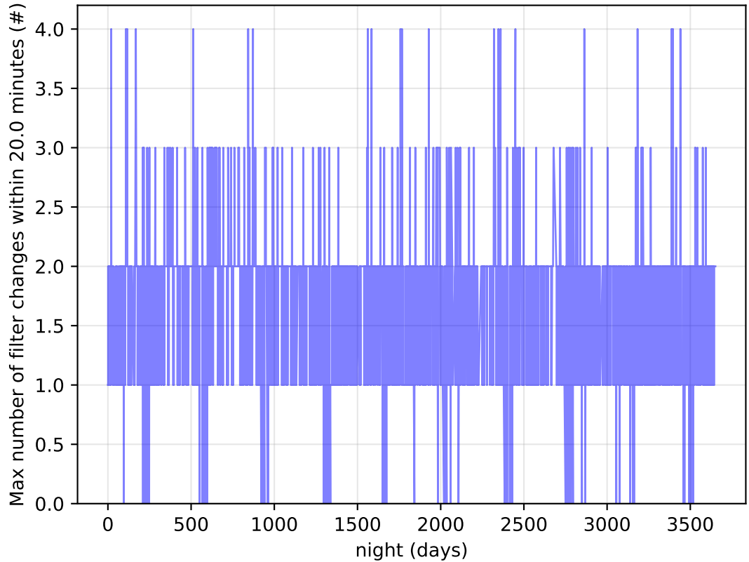
weather_cloudso14v3.4_10yrs Per Night: Max number of filter changes within 20.0 minutes
