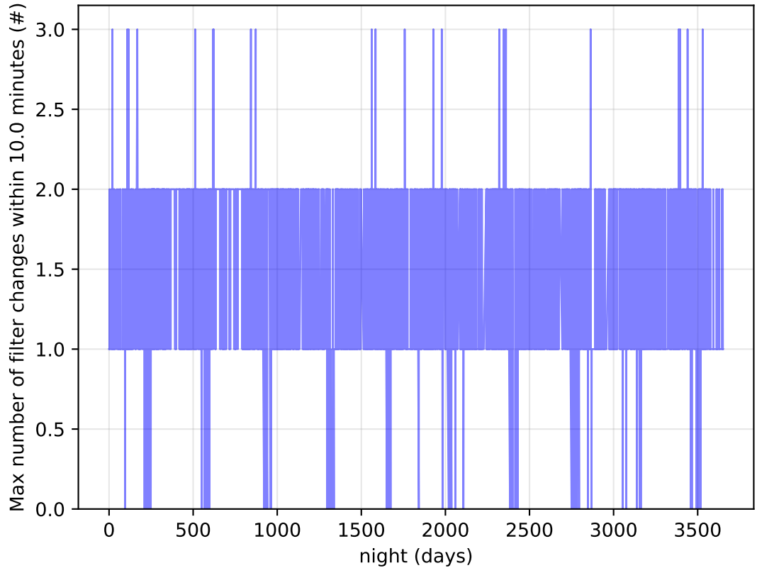
weather_cloudso14v3.4_10yrs Per Night: Max number of filter changes within 10.0 minutes
