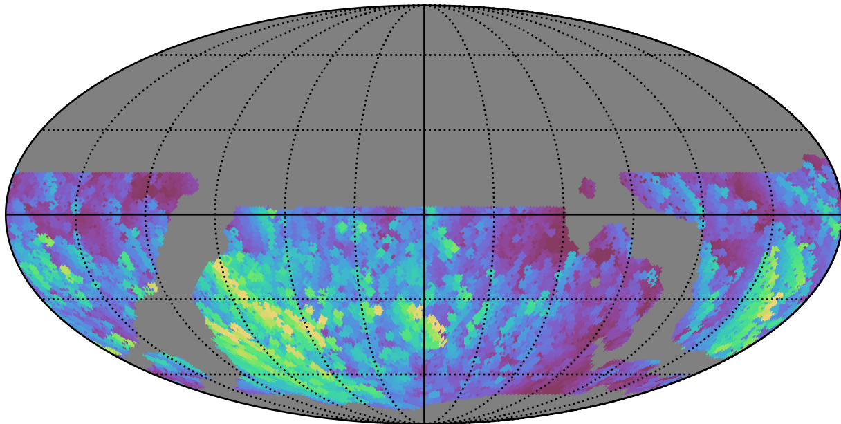
weather_cloudso14v3.4_10yrs WFD u band: Max normairmass
