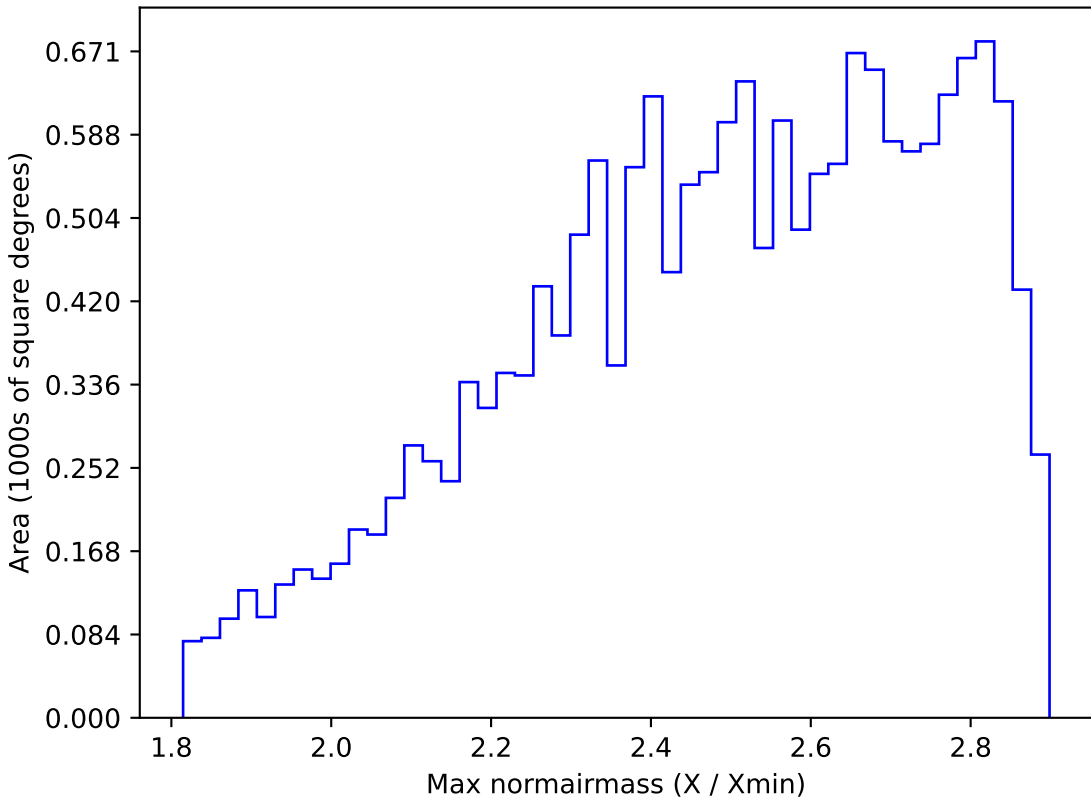
weather_cloudso14v3.4_10yrs WFD all bands: Max normairmass
