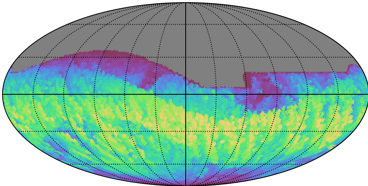
weather_cloudso14v3.4_10yrs All sky z band: Max normairmass
