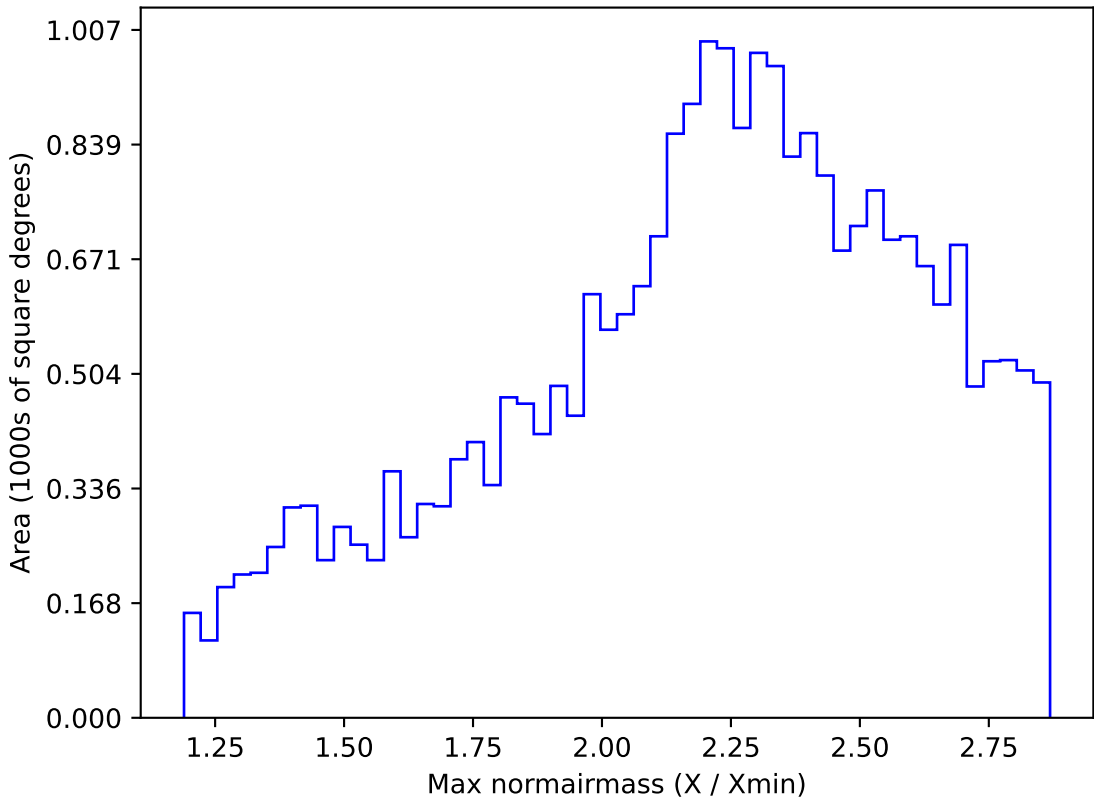
weather_cloudso14v3.4_10yrs All sky z band: Max normairmass
