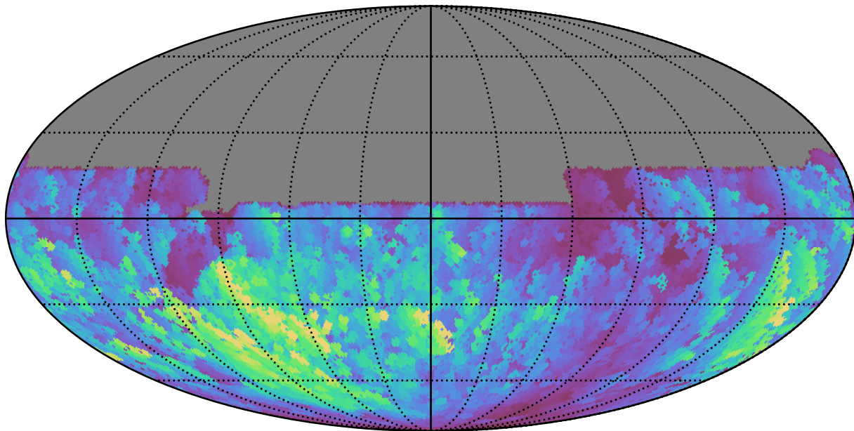
weather_cloudso14v3.4_10yrs All sky u band: Max normairmass
