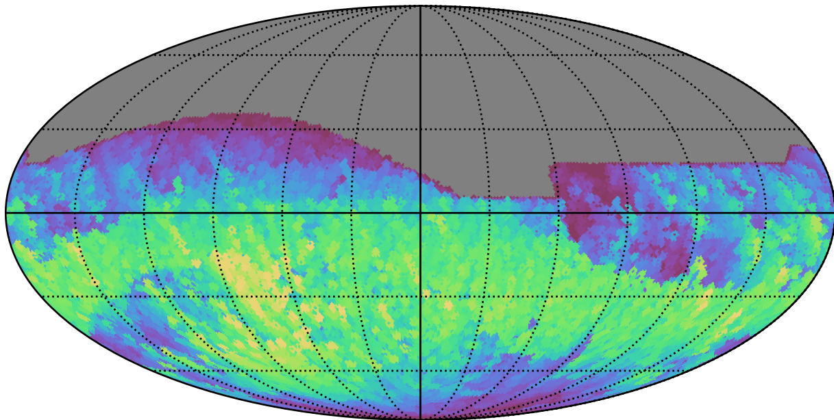
weather_cloudso14v3.4_10yrs All sky r band: Max normairmass
