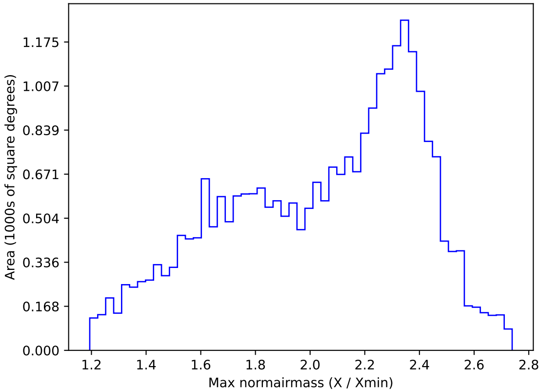
weather_cloudso14v3.4_10yrs All sky r band: Max normairmass
