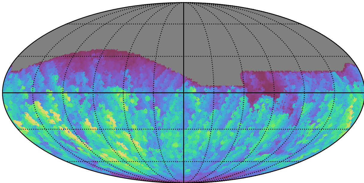
weather_cloudso14v3.4_10yrs All sky g band: Max normairmass
