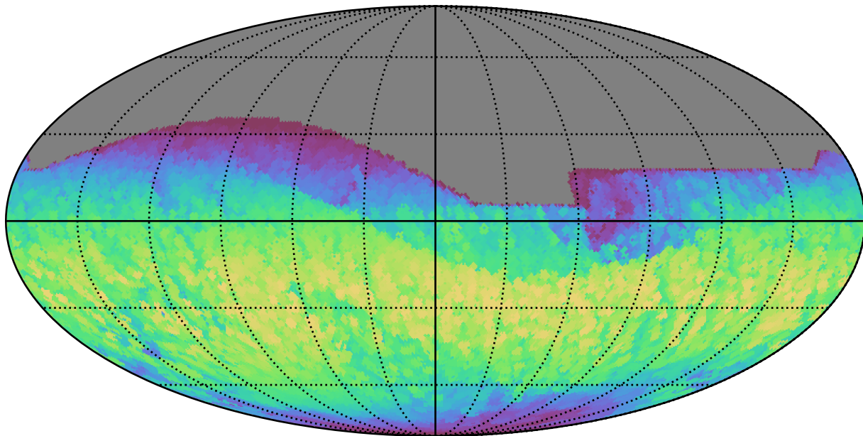
weather_cloudso14v3.4_10yrs All sky all bands: Max normairmass
