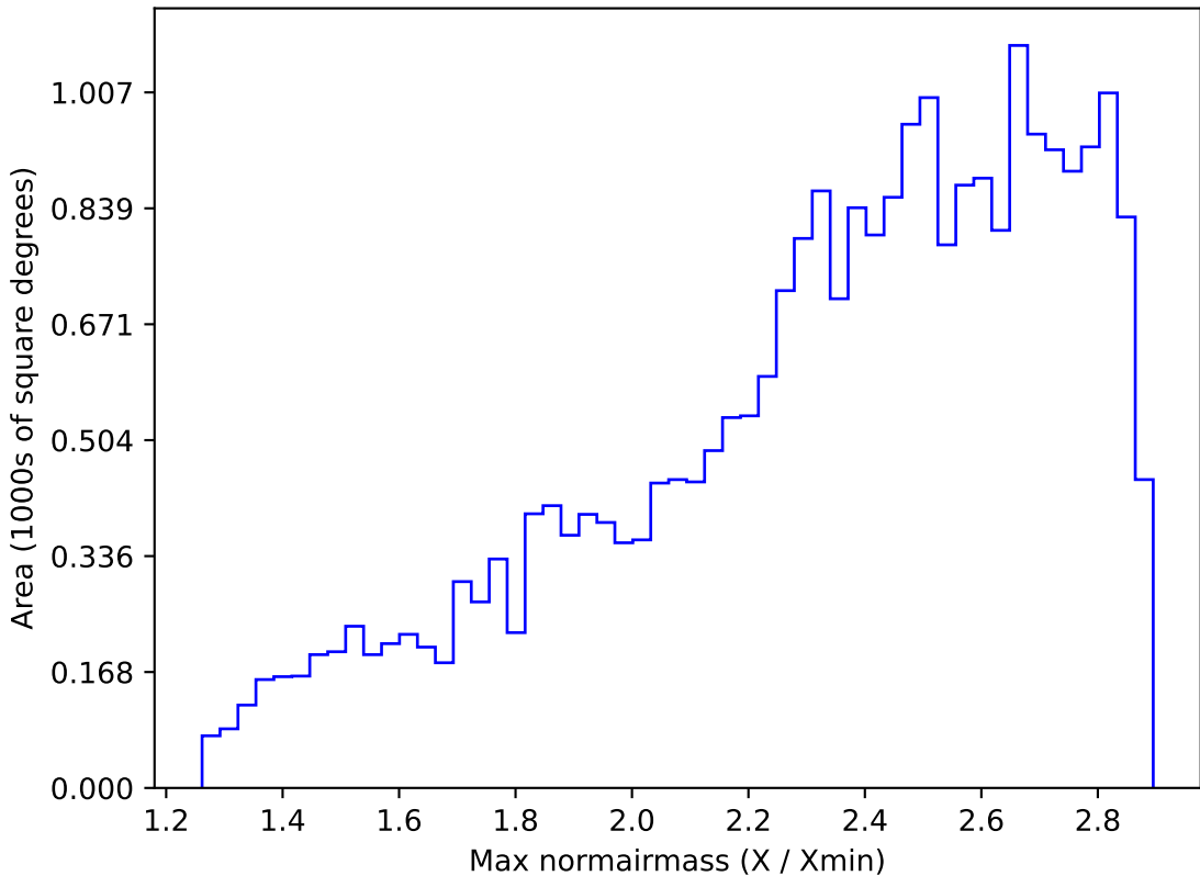
weather_cloudso14v3.4_10yrs All sky all bands: Max normairmass
