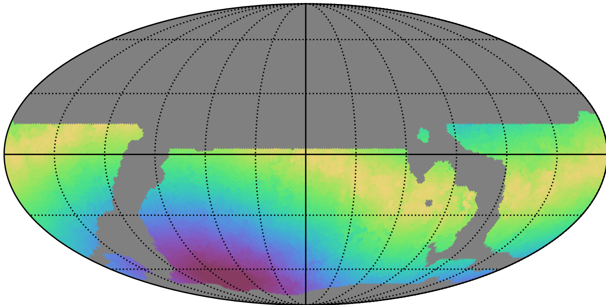
weather_cloudso14v3.4_10yrs WFD z band: Max moonDistance
