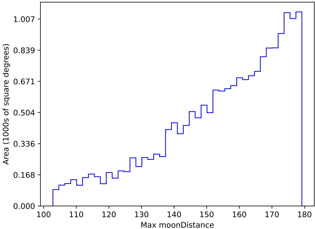
weather_cloudso14v3.4_10yrs WFD z band: Max moonDistance
