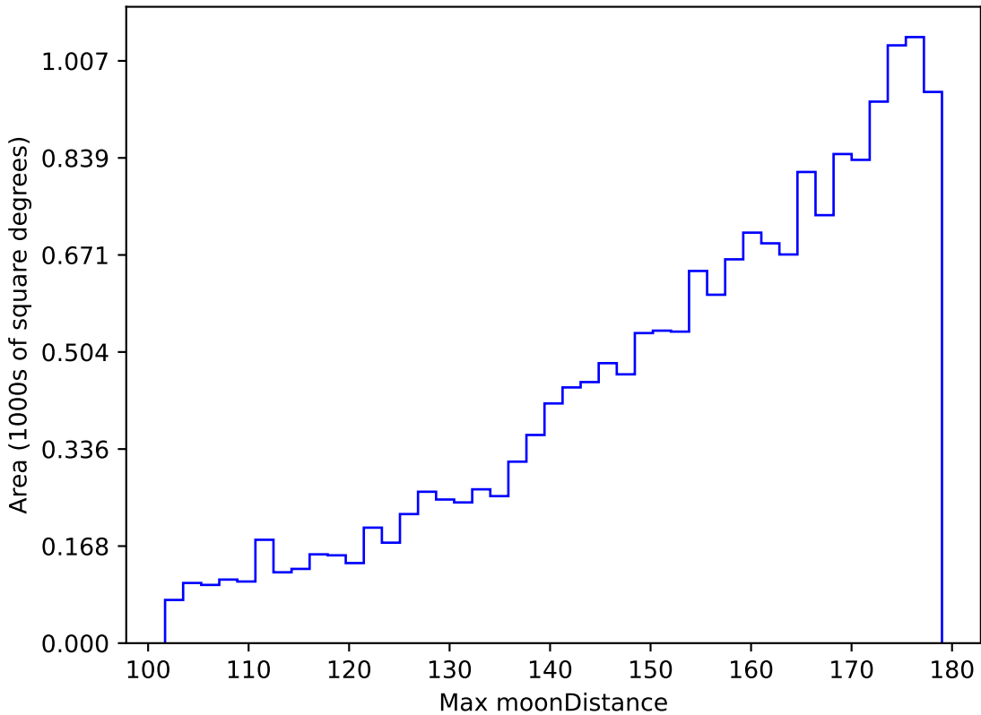
weather_cloudso14v3.4_10yrs WFD u band: Max moonDistance
