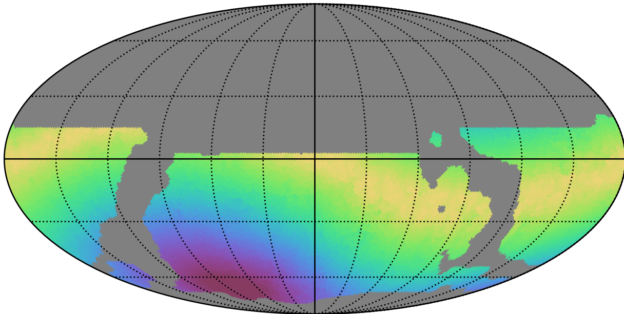
weather_cloudso14v3.4_10yrs WFD i band: Max moonDistance
