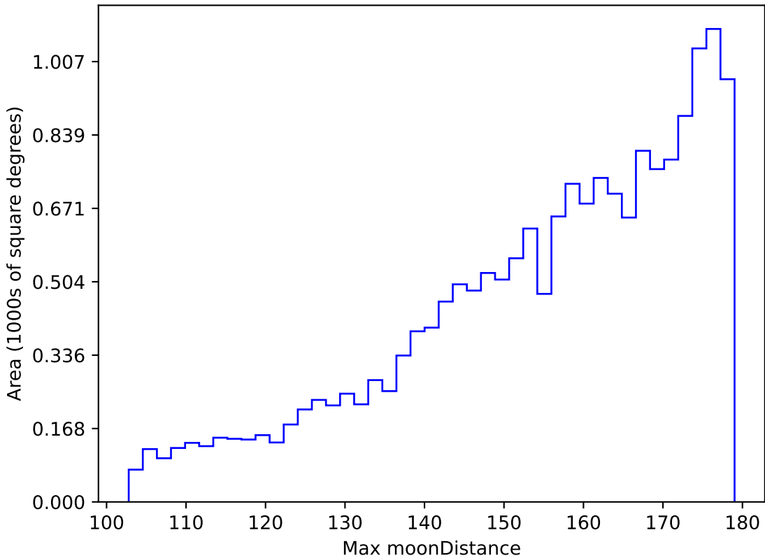
weather_cloudso14v3.4_10yrs WFD g band: Max moonDistance
