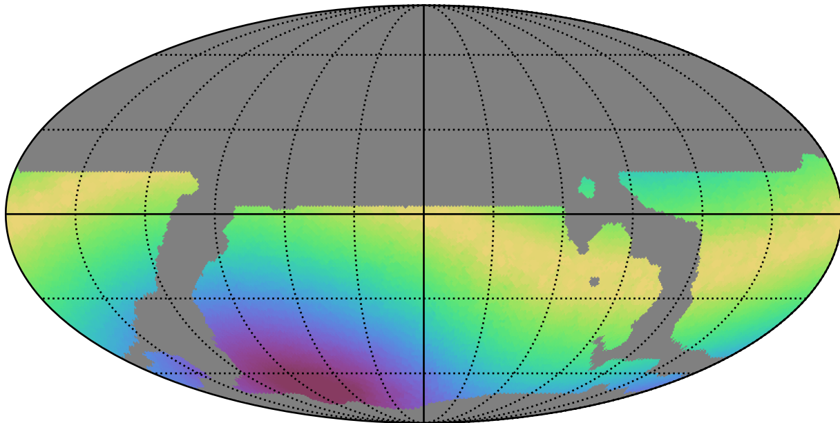
weather_cloudso14v3.4_10yrs WFD all bands: Max moonDistance
