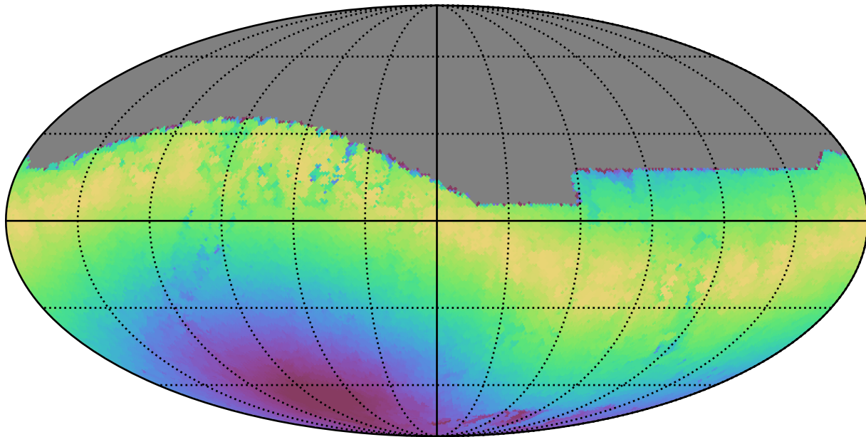
weather_cloudso14v3.4_10yrs All sky z band: Max moonDistance
