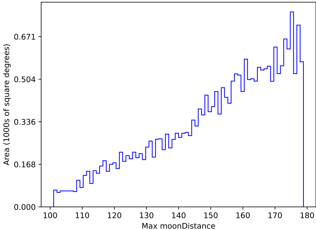
weather_cloudso14v3.4_10yrs All sky u band: Max moonDistance
