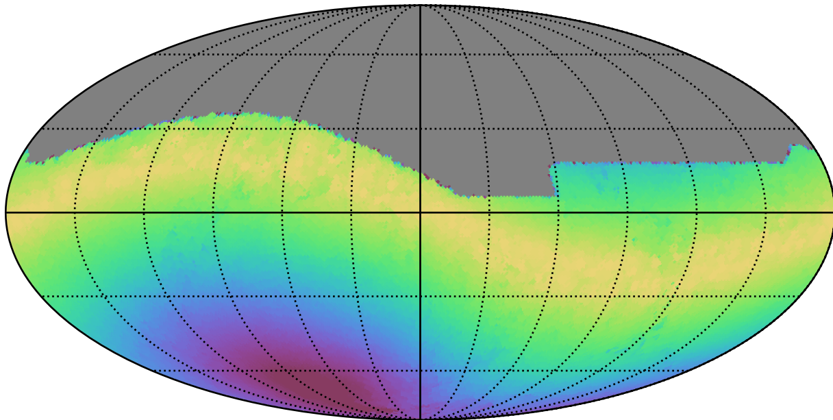
weather_cloudso14v3.4_10yrs All sky r band: Max moonDistance
