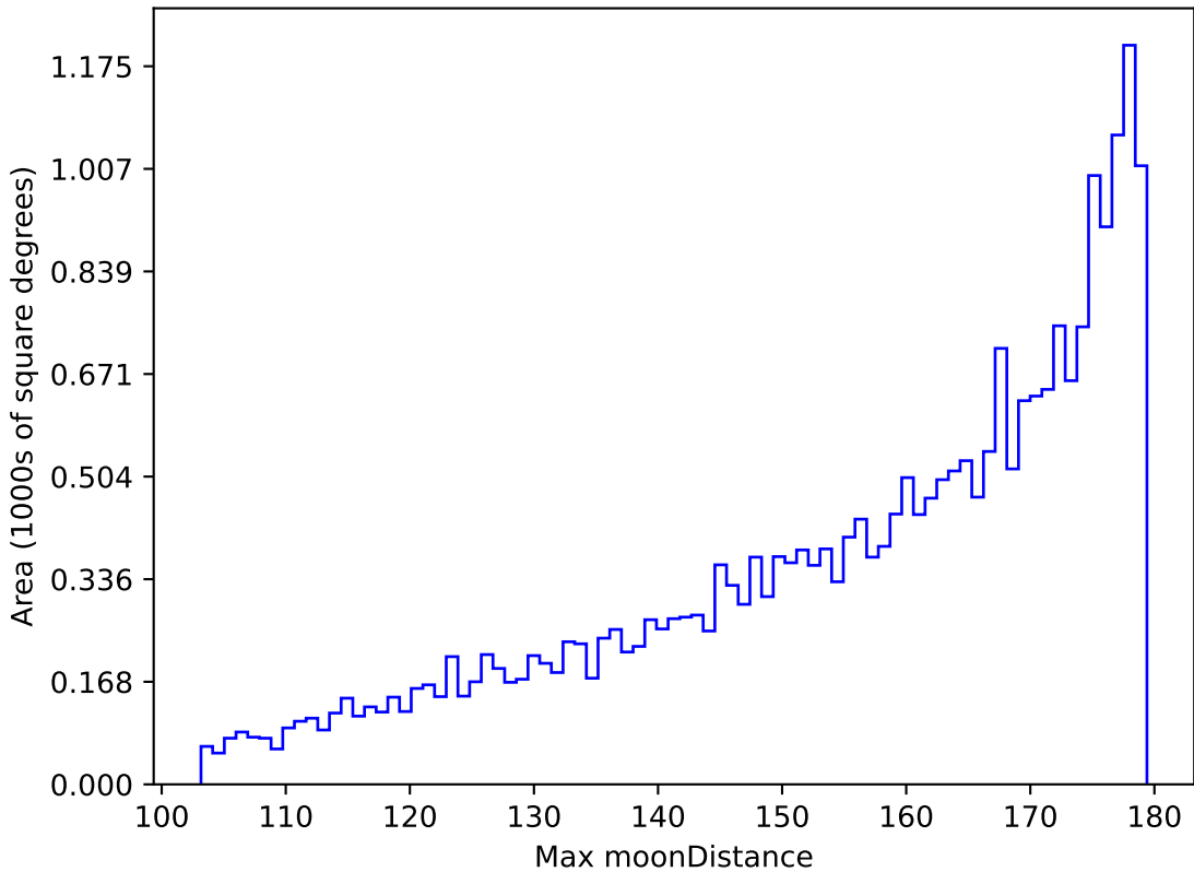
weather_cloudso14v3.4_10yrs All sky r band: Max moonDistance
