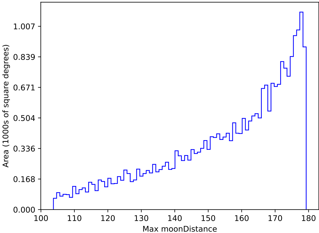
weather_cloudso14v3.4_10yrs All sky i band: Max moonDistance
