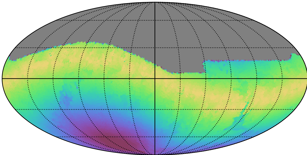
weather_cloudso14v3.4_10yrs All sky g band: Max moonDistance
