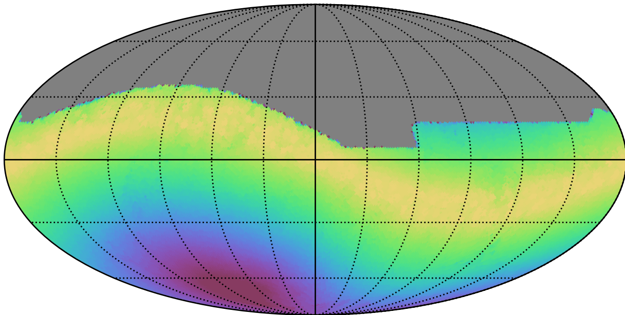
weather_cloudso14v3.4_10yrs All sky all bands: Max moonDistance
