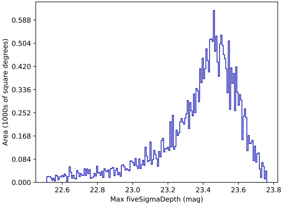
weather_cloudso14v3.4_10yrs Yr 1 z band: Max fiveSigmaDepth
