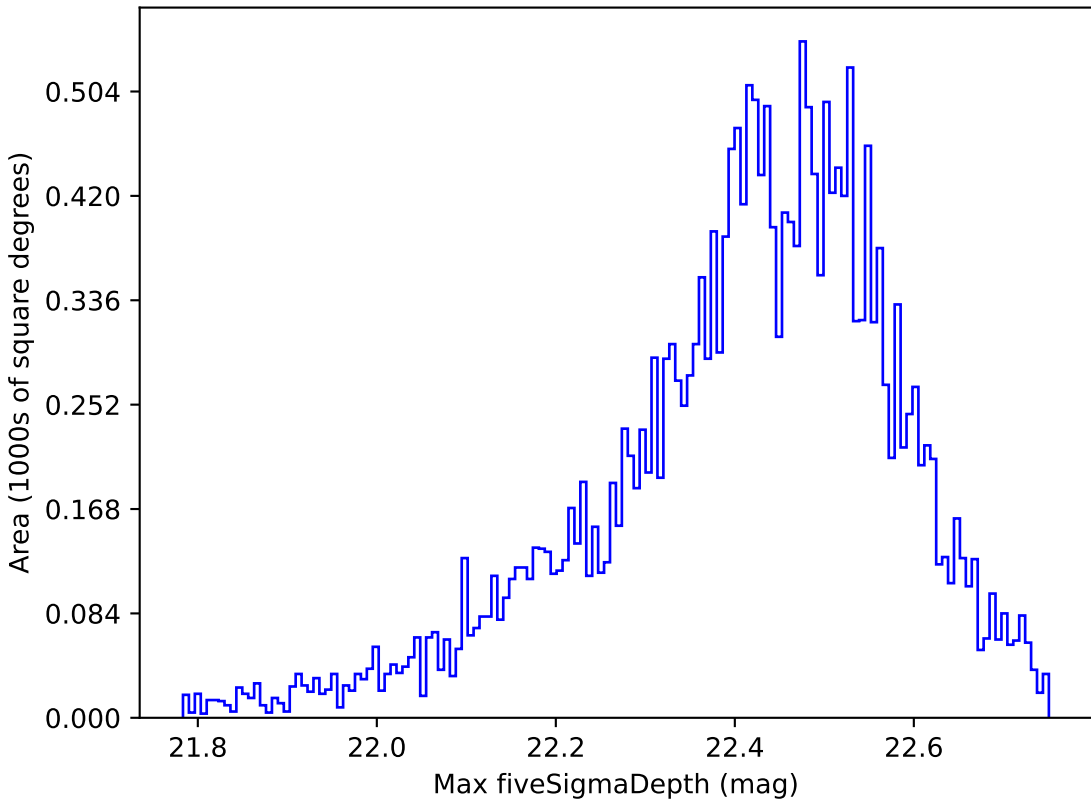
weather_cloudso14v3.4_10yrs Yr 1 y band: Max fiveSigmaDepth
