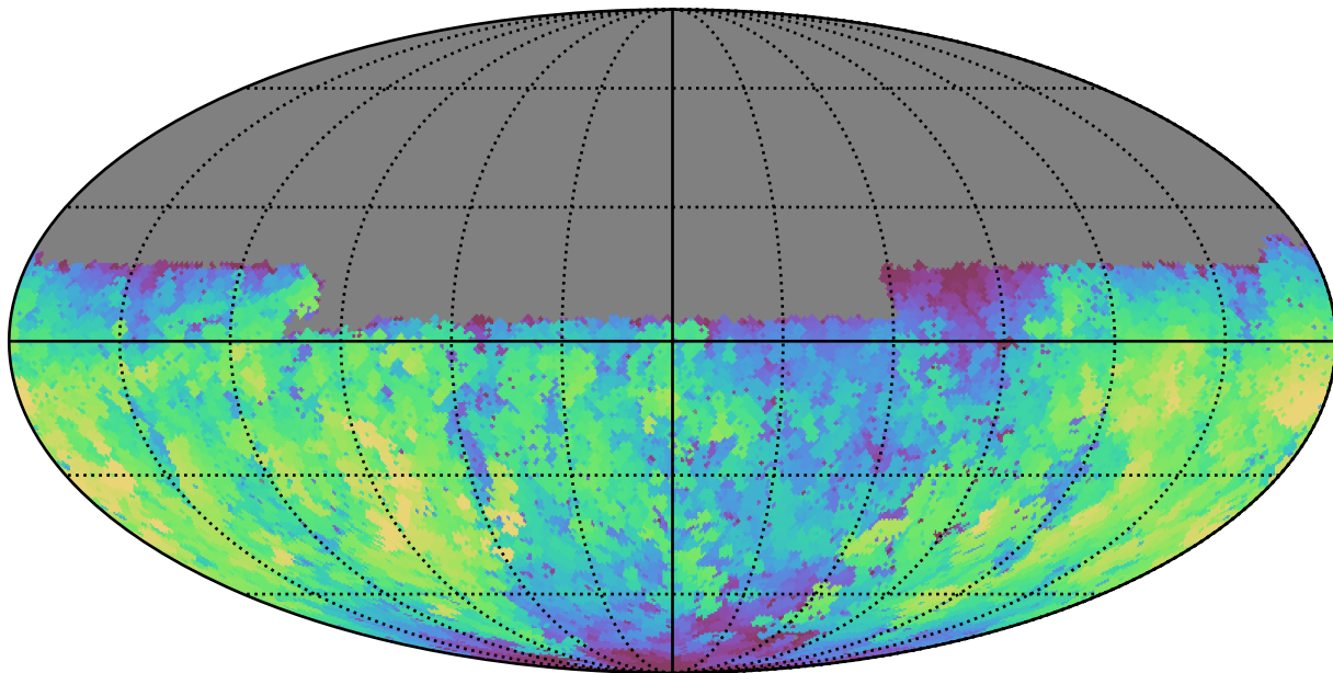
weather_cloudso14v3.4_10yrs Yr 1 u band: Max fiveSigmaDepth
