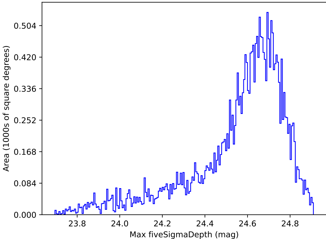
weather_cloudso14v3.4_10yrs Yr 1 r band: Max fiveSigmaDepth
