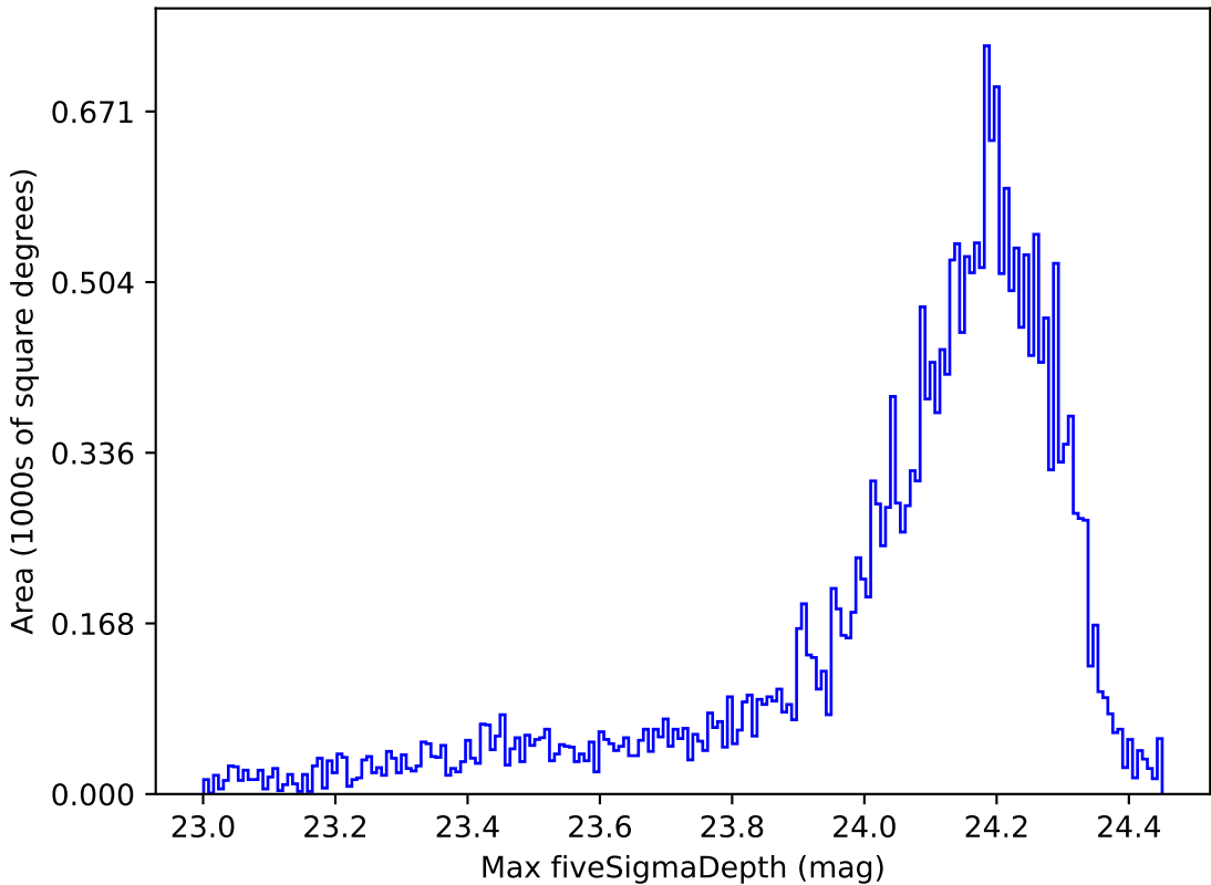
weather_cloudso14v3.4_10yrs Yr 1 i band: Max fiveSigmaDepth
