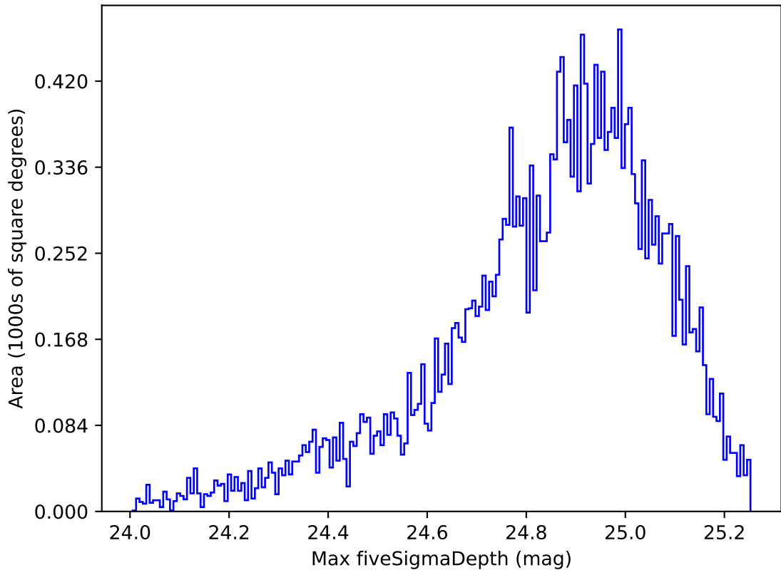
weather_cloudso14v3.4_10yrs Yr 1 g band: Max fiveSigmaDepth
