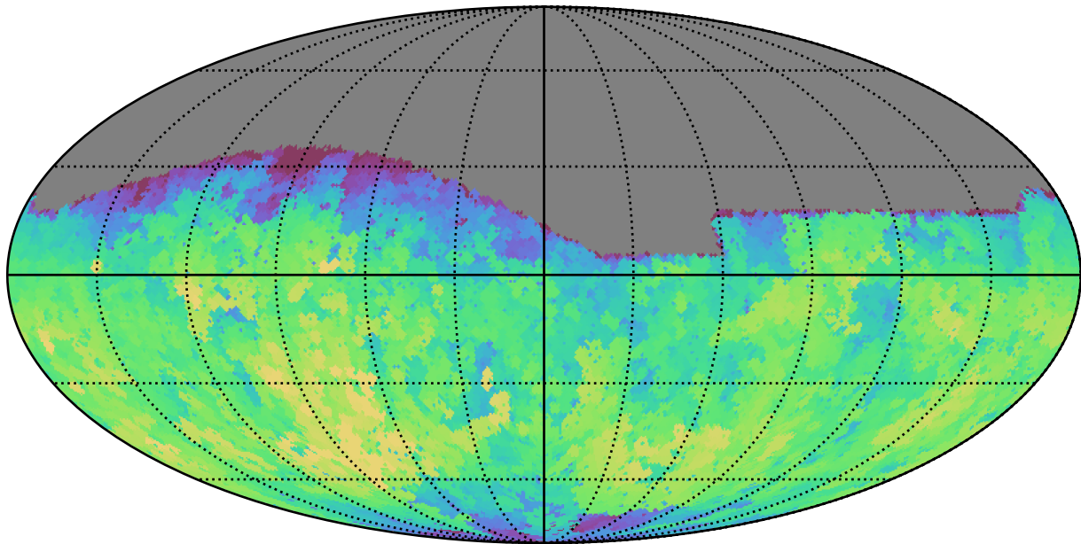
weather_cloudso14v3.4_10yrs Yr 1 all bands: Max fiveSigmaDepth
