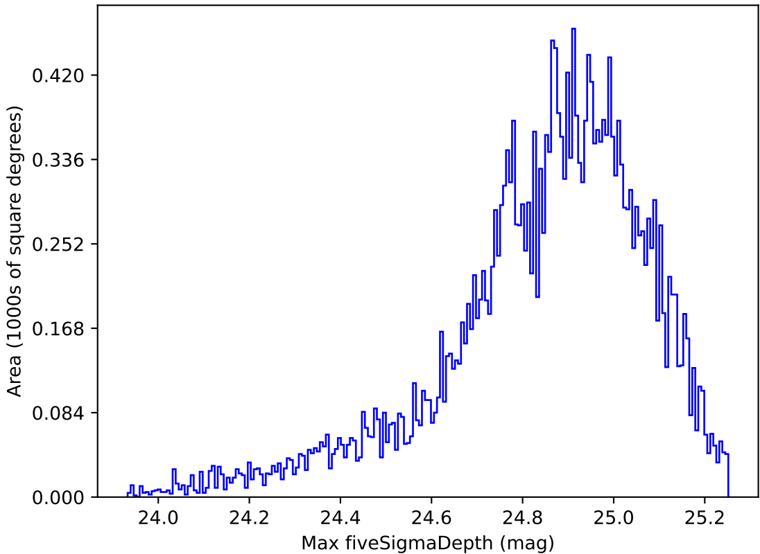
weather_cloudso14v3.4_10yrs Yr 1 all bands: Max fiveSigmaDepth
