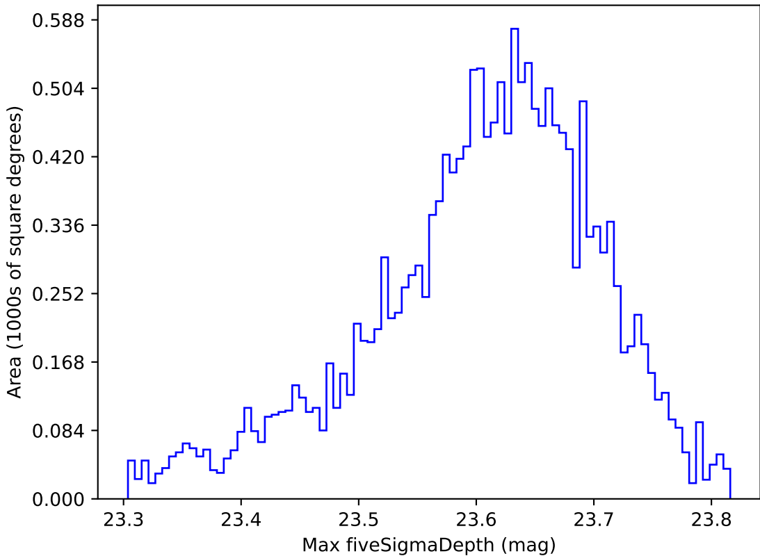
weather_cloudso14v3.4_10yrs WFD z band: Max fiveSigmaDepth
